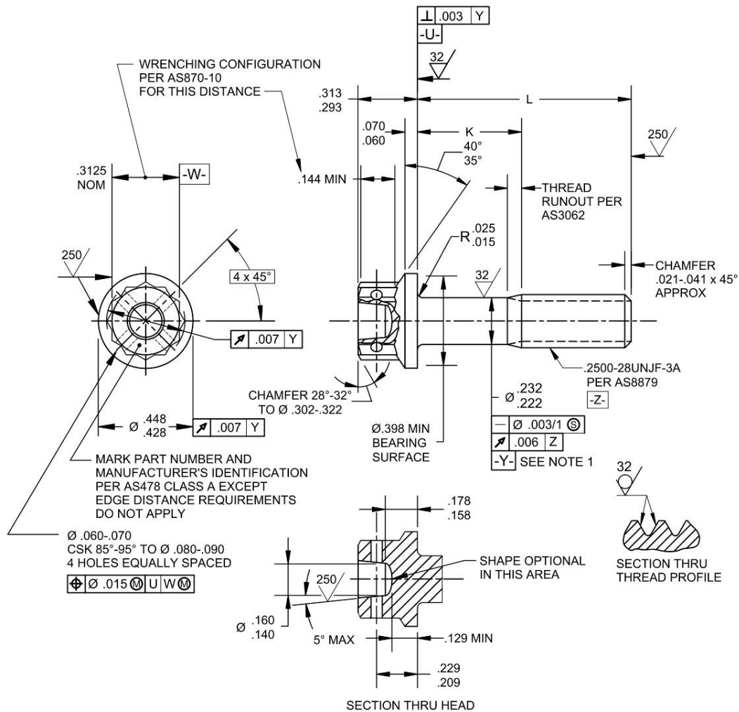
FIGURE 1 - BOLT
